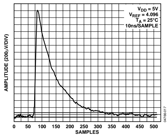
Figure 21. Glitch Energy
