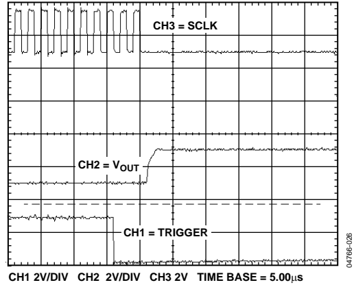
Figure 19. Exiting Power-Down
