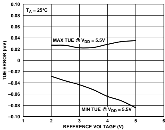
Figure 12. TUE vs. Reference Input Voltage
