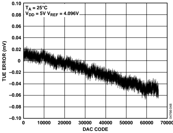
Figure 5. Typical TUE Plot
