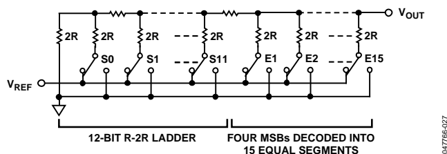
Figure 27. DAC Ladder Structure
