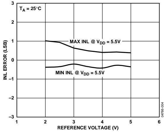
Figure 10. INL vs. Reference Input Voltage
