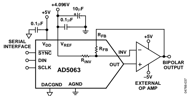
Figure 37. Bipolar Operation with the AD5063
