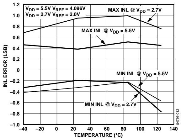
Figure 6. INL vs. Temperature
