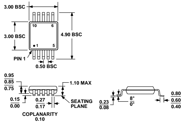
Figure 39. 10-Lead Mini Small Outline Package [MSOP] (RM-10) Dimensions shown in millimeters
