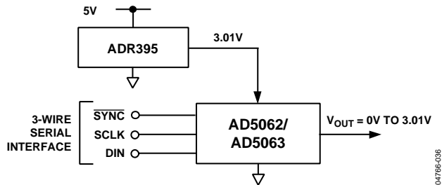
Figure 36. ADR423 as Reference to AD5063
