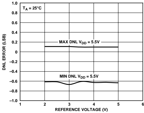
Figure 11. DNL vs. Reference Input Voltage
