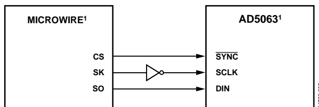
Figure 35. AD5063 to MICROWIRE Interface
